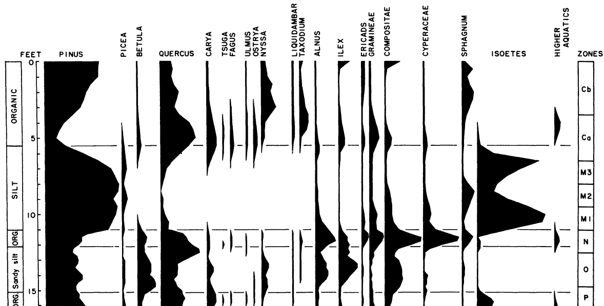
GENERALIZED POLLEN DIAGRAM FOR BLADEN COUNTY, N.C.
