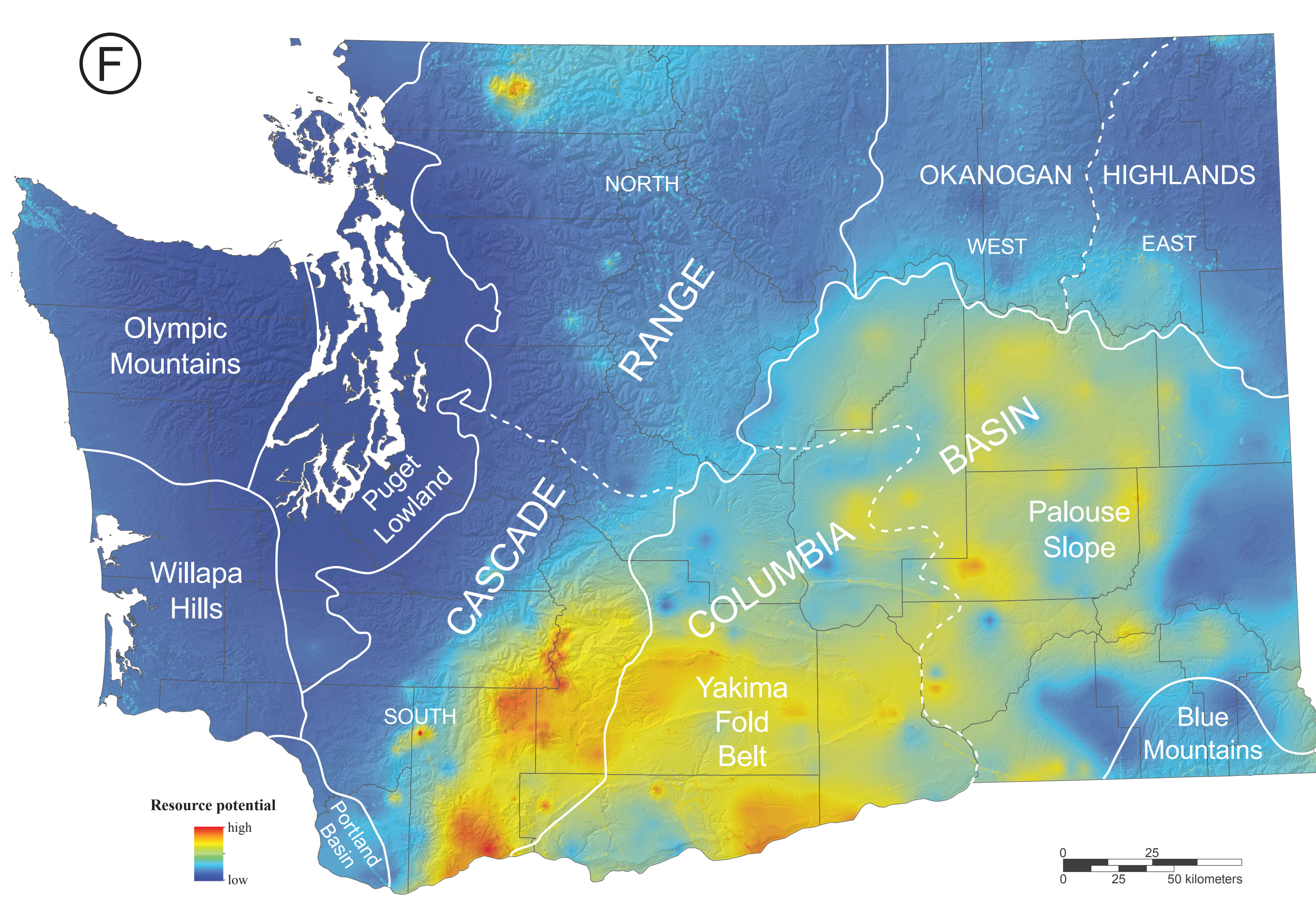
Figure F. The resource potential model represents the relative geothermal potential in Washington State based on the permeability and heat potential models. The model is intended to highlight areas of elevated potential for the presence of moderate- to high-temperature geothermal systems. This model represents geothermal resource potential without consideration of regulatory restrictions, land-management restrictions, or economic viability. The general trend of the resource potential model is similar to that of the heat potential model. Locally, areas with elevated modeled permeability potential moderately increase the relative resource potential.
