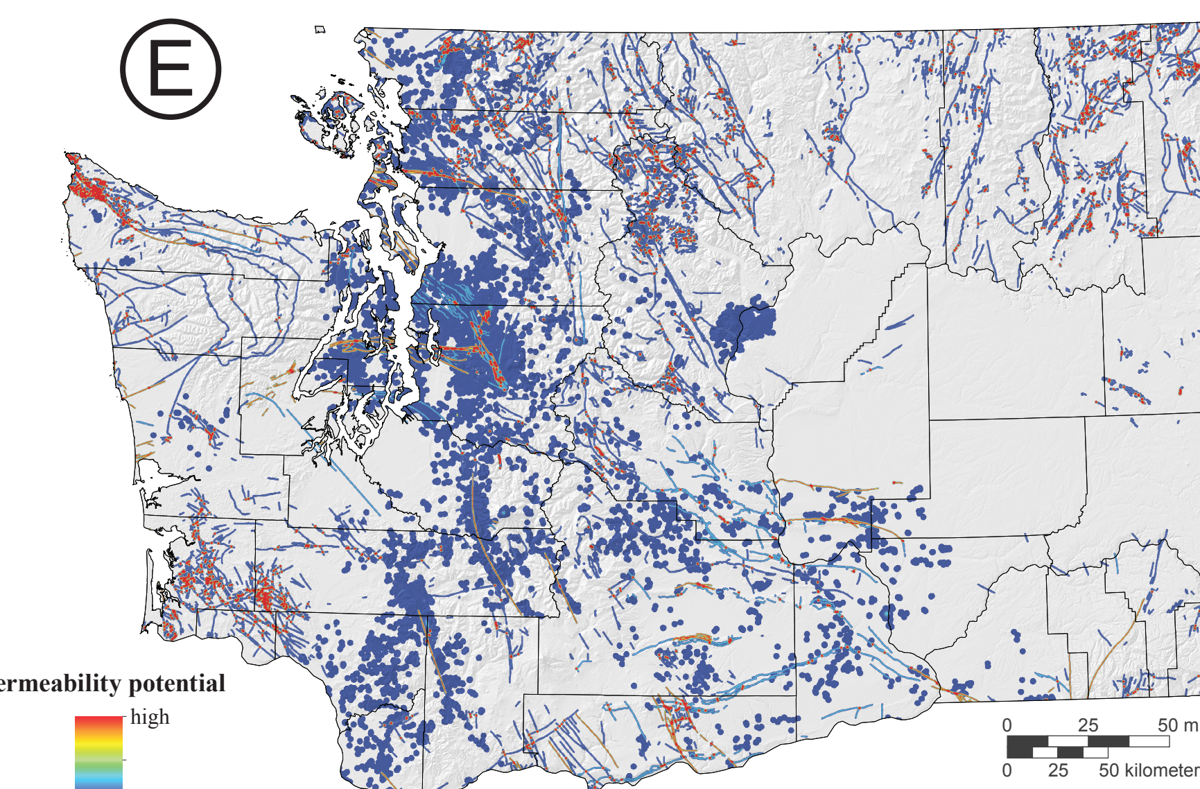
Figure E. Conventional geothermal-resource production requires significant reservoir permeability to enable thermal fluids to migrate freely through a reservoir and into the wellbores. The permeability potential model is based on the spatial distribution of known faults, fault intersections, and recorded seismic activity. The highest modeled permeability potential is found in areas of dense fault intersection, such as the northwest corner of the Olympic Peninsula and the southern Willapa Hills. Mapped fault-density variation is likely due in part to the scale and scope of fault mapping as well as the variable emphasis placed on faults by different investigators. Broad regions with recorded seismic activity are distributed widely along the western front of the Cascade Range, with isolated high-density regions across much of the state.
