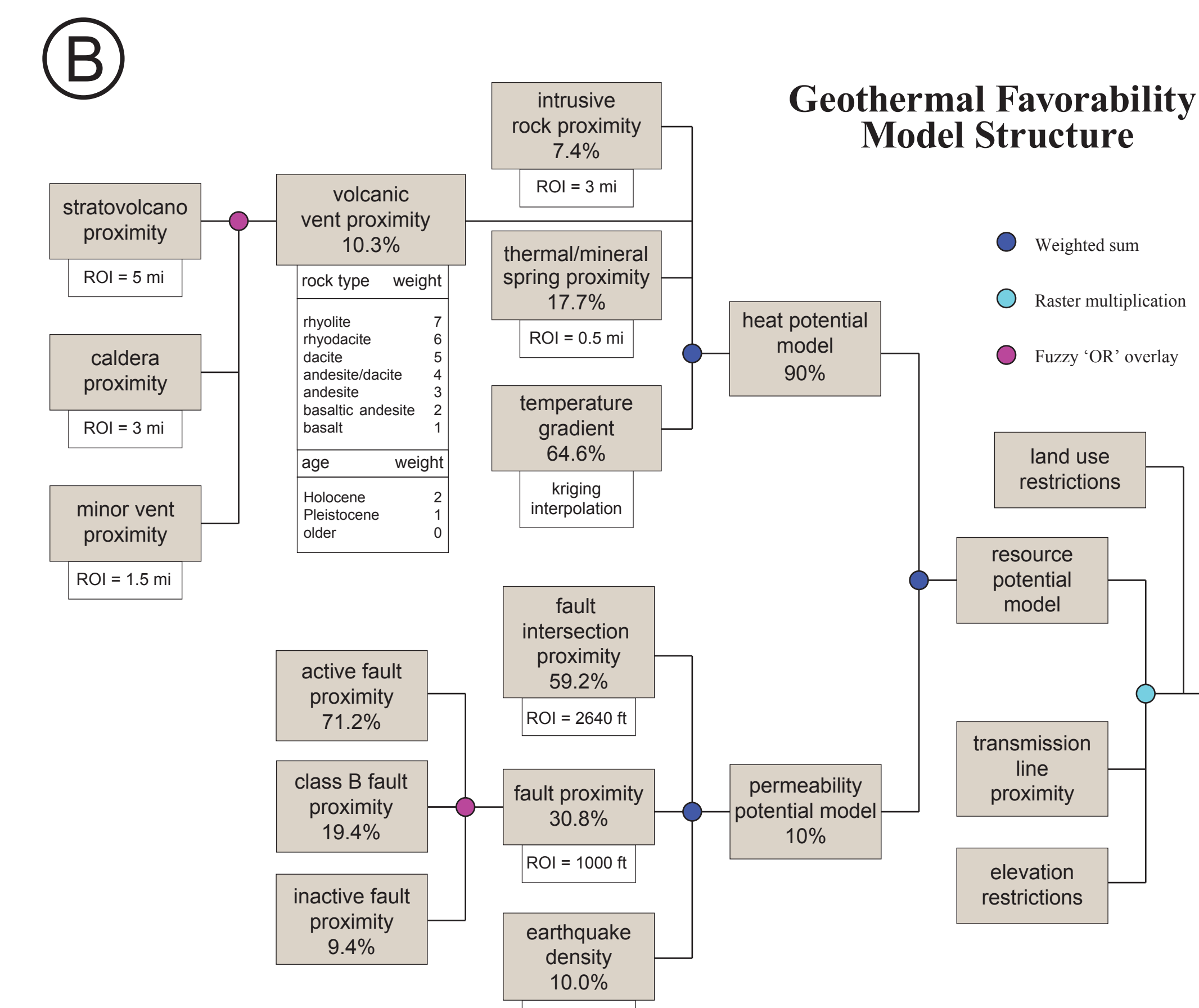
Figure B. General structure of the geothermal favorability model of Washington State, including intermediate raster data, thematic models, and favorability input models, model processes (purple, cyan, and magenta circles), classification schemes, radius of influence (ROI), and analytic hierarchy process (AHP) weights (percent). Vector input data not shown.
