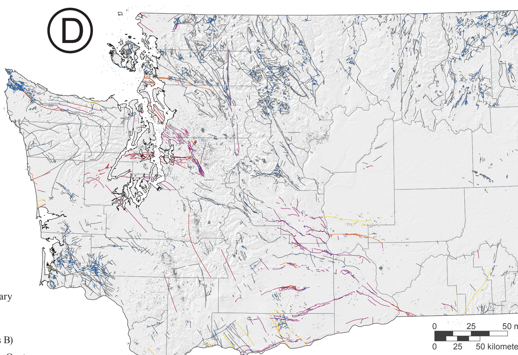
Figure D. The permeability potential model uses input data including faults, fault intersections, and earthquake locations. Fault data consist of mapped faults compiled from 1:250,000-scale, 1:100,000-scale, and active fault digital data (Washington Division of Geology and Earth Resources, 2010a; Bowman and Czajkowski, 2014). The earthquake density calculation was performed on relocated earthquakes greater than magnitude 1 and at least 30 km depth (Bowman and Czajkowski, 2014).
