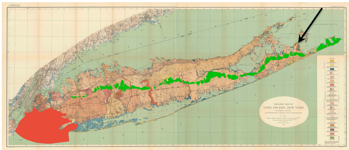
Figure 7 – Jameco Gravel and Montauk Till. The Jameco Gravel (red overlay) is an outwash sand mapped in western Long Island, and is usually considered Illinoian age. Fuller's Montauk Till is mapped in eastern Long Island in the general vicinity of, and below, the Ronkonkoma moraine (green overlay). See arrow – brown map unit is too small to see clearly at this scale. Slivers of it are also exposed by coastal erosion along the north shore of Long Island. This stratum is also generally considered to be Illinoian age. (Modified from Smolensky & Others (1989) and Fuller (1914).)
