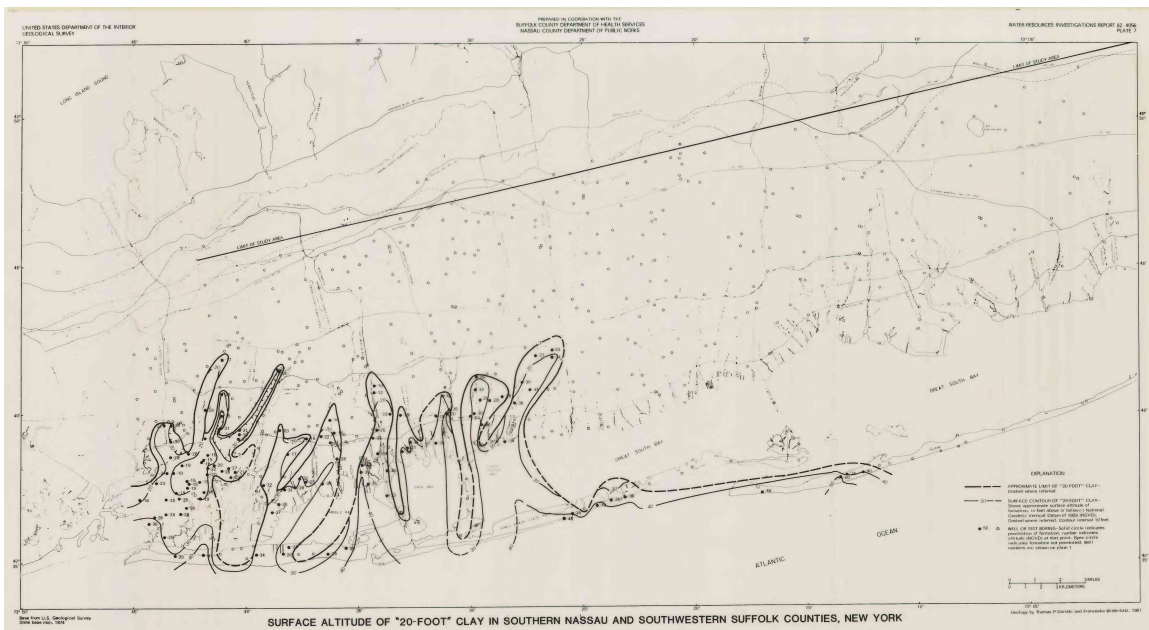
Figure 3 – Doriski & Wilde-Katz (1983) maps the presence and surface contours of the 20-Foot Clay in Nassau and Suffolk counties in Long Island. The 20-Foot Clay is an interglacial or interstadial marine clay within the Upper Glacial Aquifer. It is likely the same stratum as Fuller’s Vineyard Formation.
