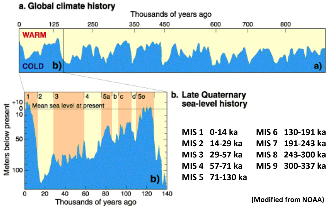
Figure 13 – Estimated global Pleistocene sea-level. The sediments that make up the 20-Foot Clay/Wantagh Fm. are typically deposited at or fairly close to sea-level. The last time sea-level was estimated to be within 20 feet (~6 meters) of the current level was during MIS5e, roughly 120,000 years ago. The region would have had to have been isostatically depressed to a significant extent, roughly 75 meters, during MIS 3 to approach the estimated sea-level. The ages associated with the more recent Marine Isotope Stages are shown in the lower right corner. (Modified from NOAA, National Climatic Data Center website, MIS ages obtained from Lisiecki & Raymo, 2005.)
