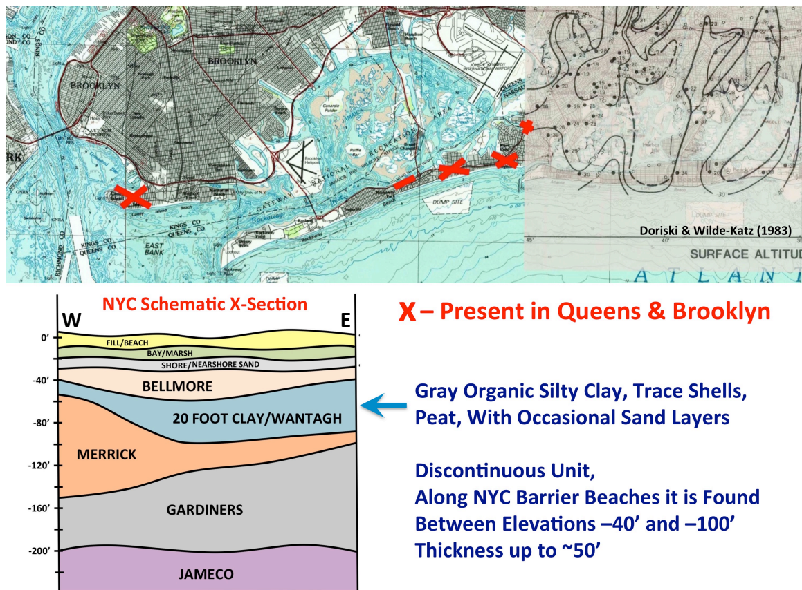
Figure 4 – Data in MRCE archives confirms that the 20-Foot Clay is a discontinuous unit that extends westward into Queens and Brooklyn. Red X's show locations where its presence is confirmed. The schematic W-E cross-section below the NYC shoreline is very simplified, but it illustrates how the clay, in places 50' thick, can be a significant stratum that should be taken into consideration in a subsurface investigation. Rampino & Sanders (1981) renamed the stratum the Wantagh Formation and named the sand layers usually found below (Merrick Fm.) and above it (Bellmore Fm.). In USGS publications these 3 formations are usually just grouped together as part of the Upper Glacial Aquifer. (Modified from Doriski & Wilde-Katz (1983) and USGS Long Island West (1984) and Newark (1986) quadrangles.)
