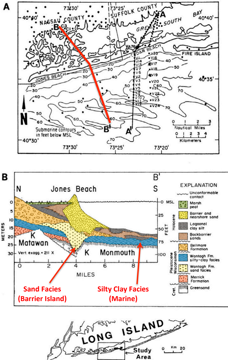
Figure 5 – Rampino & Sanders (1981) studied the 20-Foot Clay and surrounding strata in greater detail in the vicinity of Jones Beach, renaming the unit the Wantagh Formation. Cross-section B-B' shows the strata in a N-S onshore-offshore direction. The Wantagh's silty-clay facies is the marine clay portion of the stratum, the sand facies is barrier island sand within it. The Merrick outwash? is found below, and the Bellmore LGM outwash lies above the Wantagh. (Modified from Sanders & Merguerian 1997.)
