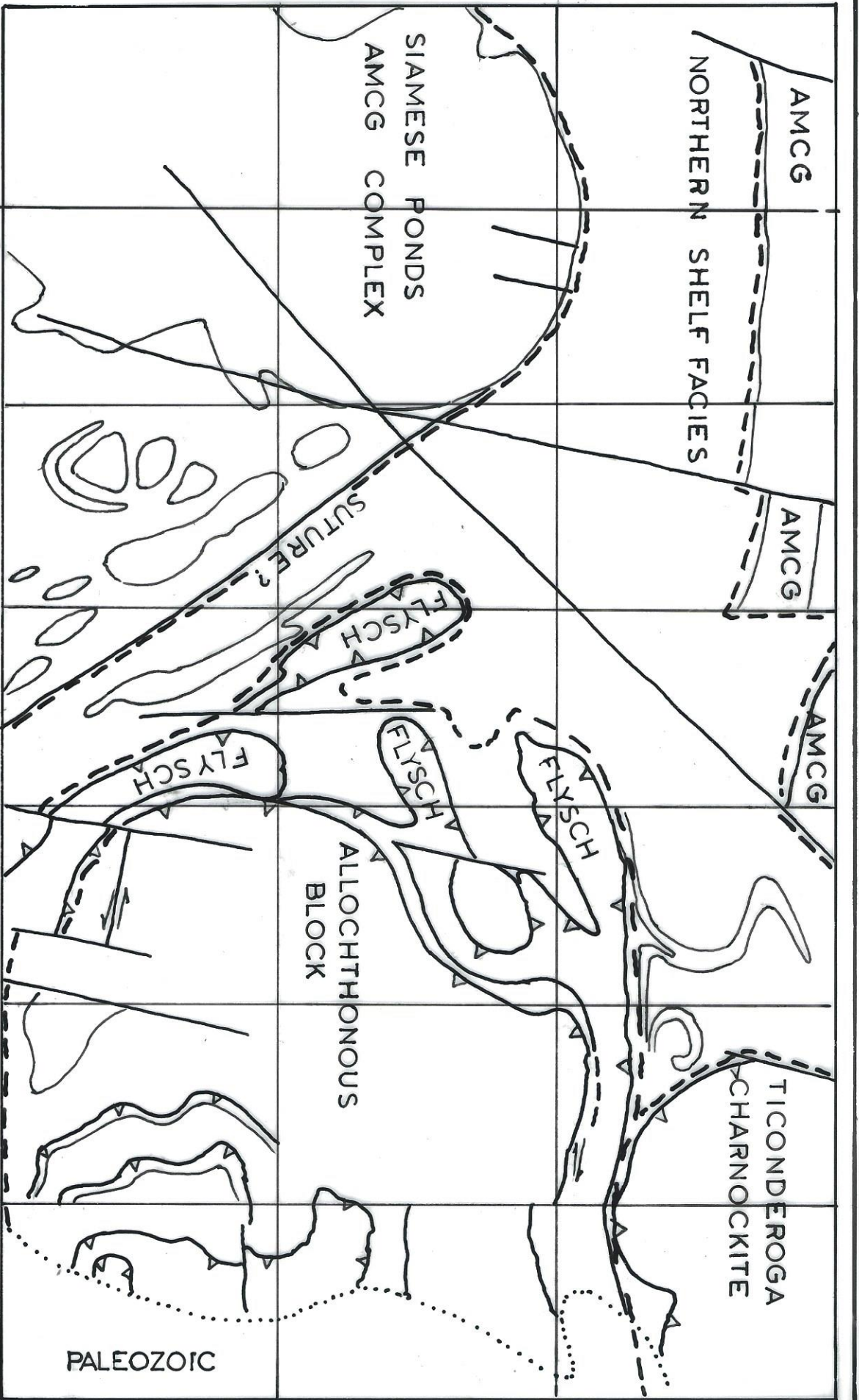
MAJOR GEOLOGICAL SUBDIVISIONS, SOUTH CENTRAL TO SOUTHEASTERN ADIRONDACK MOUNTAINS, NY
